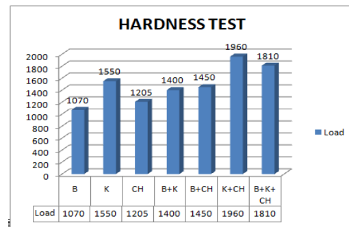
Graph 4Hardnessnumber resultgraph
