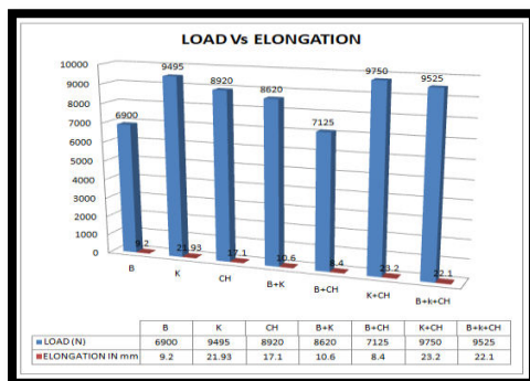
Graph 1 tensiletestresultgraph
