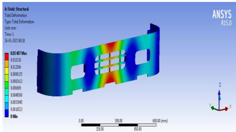
Figure 34 Total deformations of Kevlar fiber + 10grms Horn powder Material
